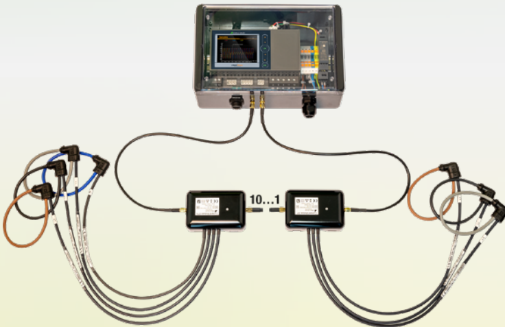
MULTIFUNCTIONAL POWER QUALITY ANALYZER FOR SMART GRID APPLICATIONS – SCALABLE LINAX PQ5000CL
